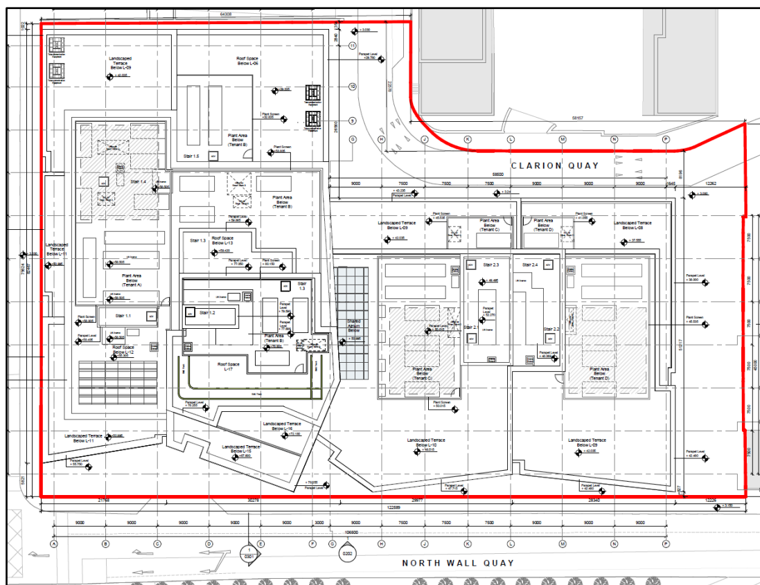
Figure 4.2 Proposed Site Layout for the Proposed Development (HJL 1NWQ-HJL-AX-17-DR-A-0117)
